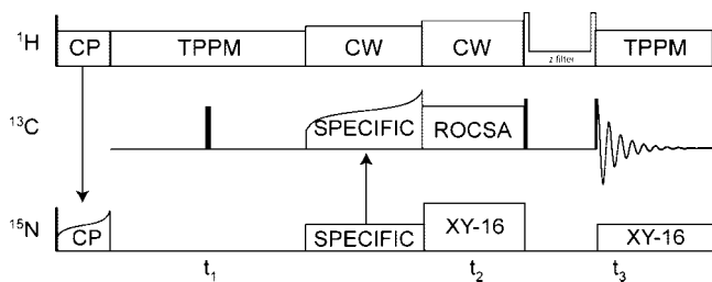
Figure 1. ^{15}\text{N} - ^{13}\text{C} CSA- ^{13}\text{C} 3D ROCSA pulse sequence. Transverse ^{15}\text{N} coherence is created by adiabatic CP from ^1\text{H} , followed by isotropic chemical shift evolution period ( t_1 ) and selective polarization transfer to ^{13}\text{C}\alpha with SPECIFIC-CP. 27 ROCSA 25 recoupling is applied to the ^{13}\text{C} spins, with a coherence filter (including States-TPPI hypercomplex sampling) prior to acquisition. During ^{13}\text{C} ROCSA, ^1\text{H} was decoupled with a CW field ( \sim 125 kHz nutation frequency) and ^{15}\text{N} with rotor-synchronized \pi -pulses of 10 \mu\text{s} with XY-16 supercycling.
